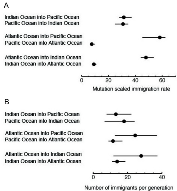
Figure 4 Estimates of gene flow for bigeye tuna populations among ocean basins based on Bayesian inferences of migration rates and population sizes. Dots are the maximum posterior values, and the lines show the 95% credibility intervals. (A) Mutation scaled immigration rate, M , between ocean basins. M is the ratio of immigration rate and mutation rate. (B) Number of immigrants per generation, N_m . 95% confidence intervals are shown.
