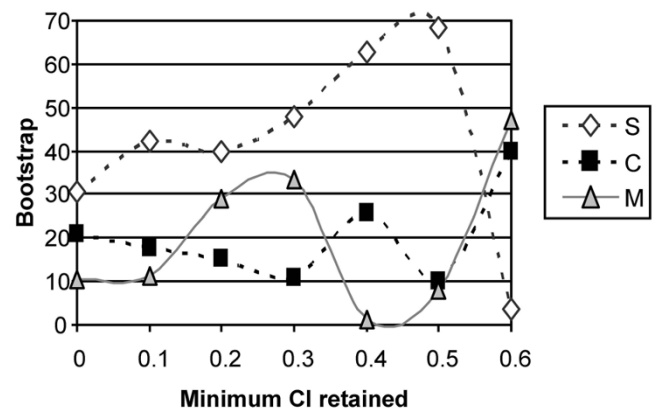
Figure 3 Bootstrap support as a function of the minimum CI of sites retained in the data. S: the best topology with the squirrel-related clade at the base of the rodent tree; M: the best topology with the mouse-related clade at the base of the rodent tree; C: the best topology with Ctenohystrica at the base of the rodent tree. Seven datasets were considered: (1) all sites (6,255 bps; CI range 0.0625–1); (2) sites with CI > 0.1 (6,210 bps); (3) sites with CI > 0.2 (5,864 bps); (4) sites with CI > 0.3 (5,432 bps); (5) sites with CI > 0.4 (4,833 bps); (6) sites with CI > 0.5 (4,119 bps); and (7) sites with CI > 0.6 (4,023 bps).
